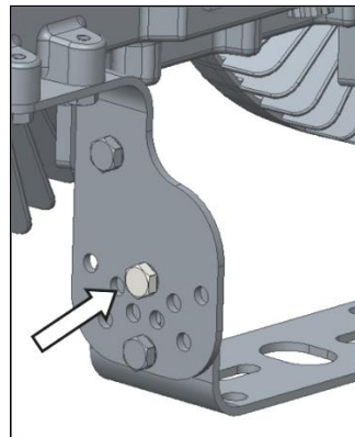
Figure 1 - Pivot Bolt
