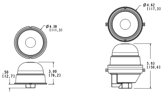
Retro-fit Unit
