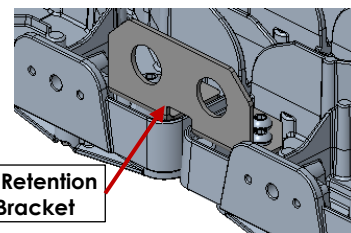
Slip Filter Base Retention Bracket
