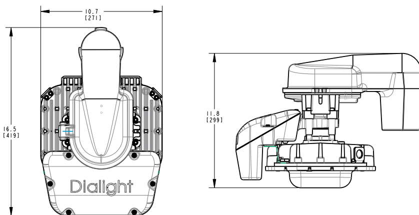
45° Wall Mount
