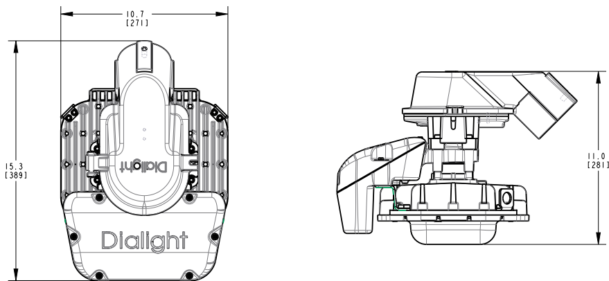
45° Stand-on Mount
