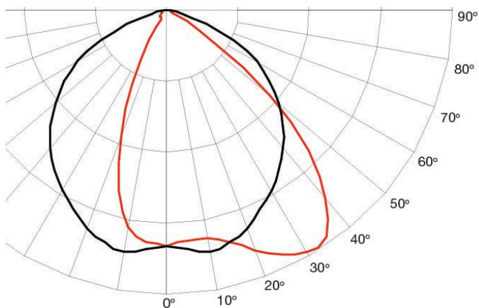
180° Beam Angle
