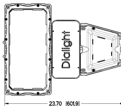
(F/S)1 MAST ARM
