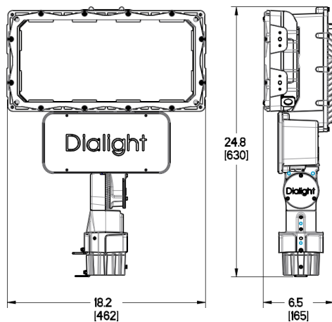
(F/S)1 SLIP FITTER - UL 844
