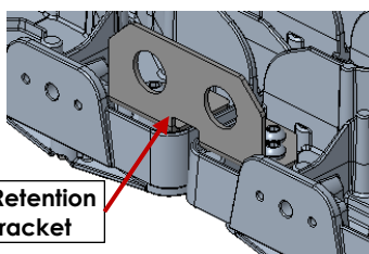
Slip Fitter Base Retention Bracket
