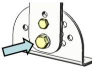
Drehmoment = 34 N-m (25 ft-lb)
